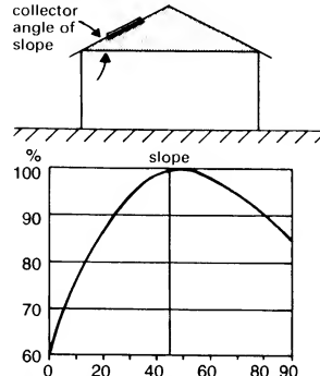
⑥ Angle of slope of collector
